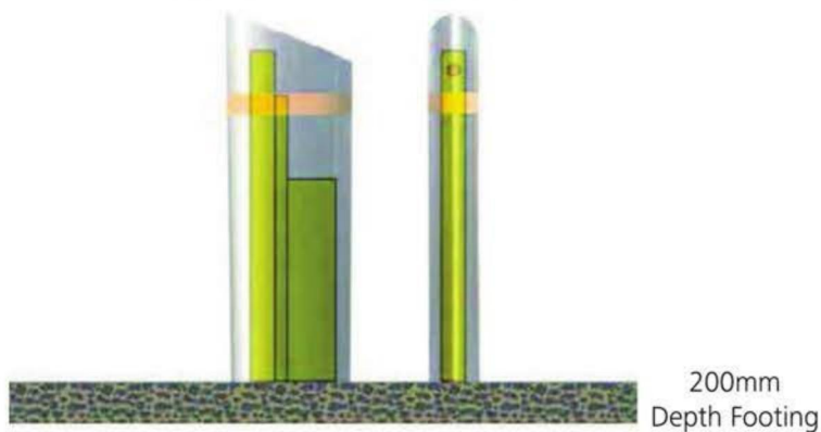
Spring Bollard Cover Side View
