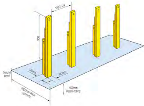
Spring bollard arrangement
