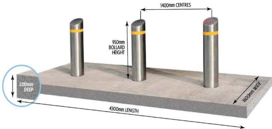
FOUNDATION SIZE FOR THREE BOLLARD RUN
